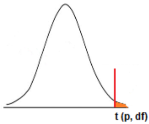
Right-sided T-distribution table
